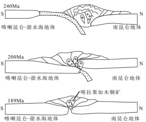
图9 喀拉果如木铜矿成矿地球动力学模式图 Fig.9 Schematic diagrams showing the formation of Kalaguorumu Cu deposit
