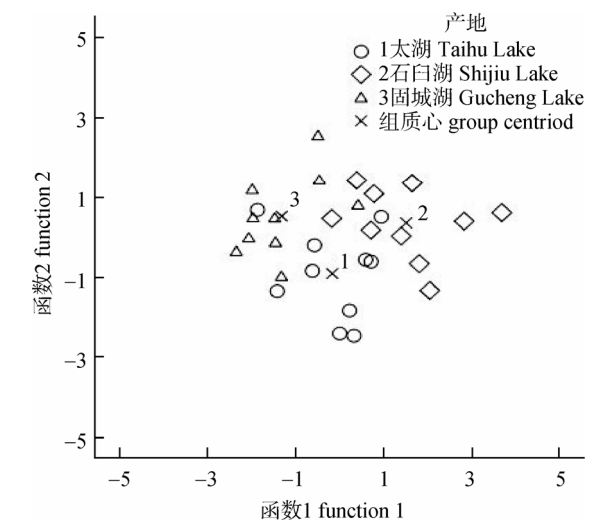
图 3 3 个湖泊产中华绒螯蟹样本形态判别分析散点图 Fig. 3 Canonical plot scores from discriminant analysis on morphological measurements of Eriocheir sinensis from three different lakes
